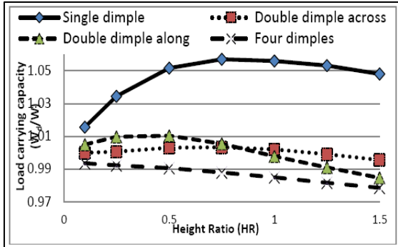
Fig. 12 Coefficient of Friction Ratios Versus Height Ratios for Multi Texture
